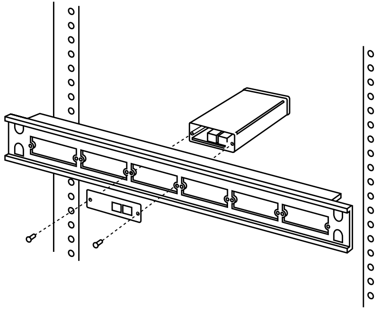
Figure 1. Rackmounting a Local or Remote Module (Dual Remote Module shown, with left side facing forward).
