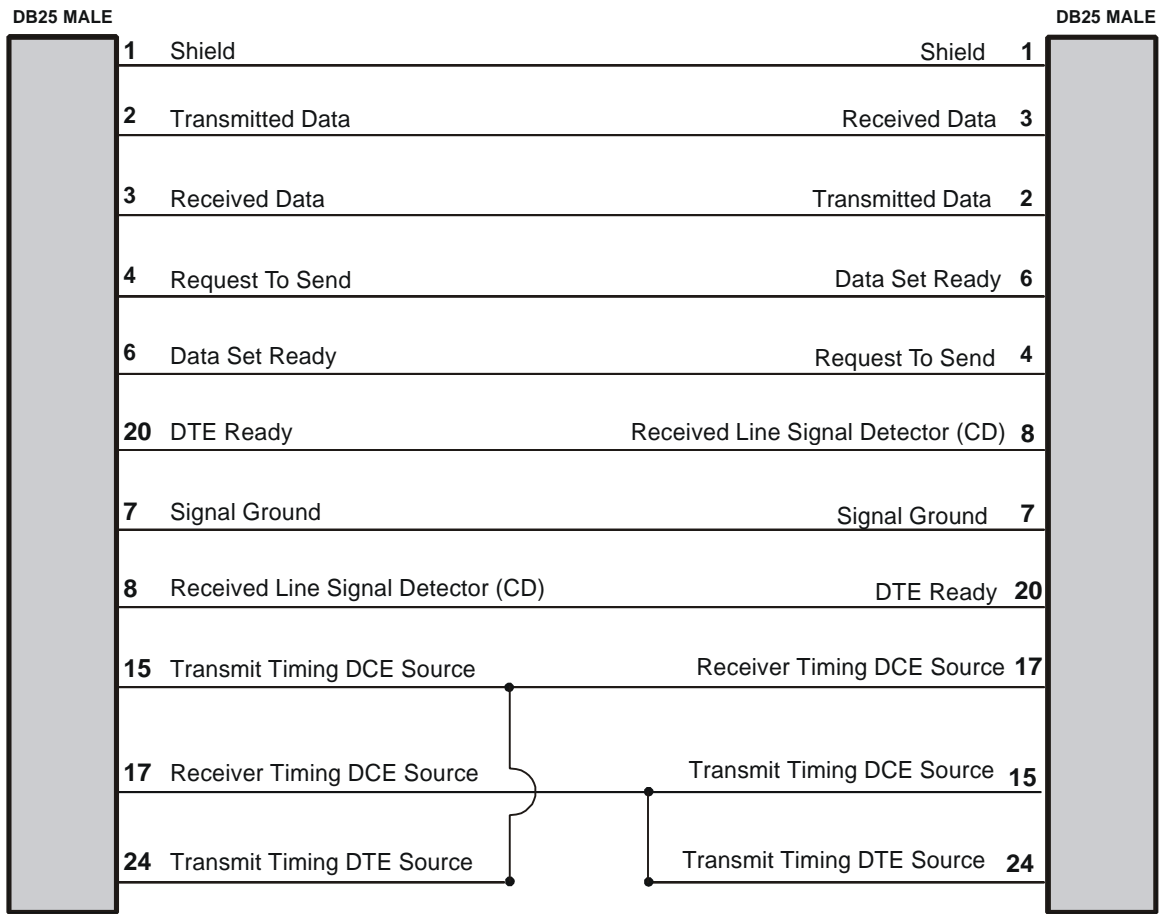
Figure 3 - 11 RS232 Null-Modem Cable
