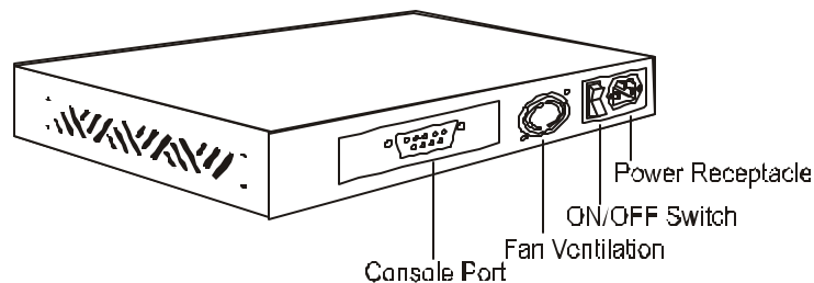
Figure 1: Rear view
