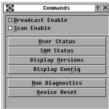
Figure 4-13. Commands window
