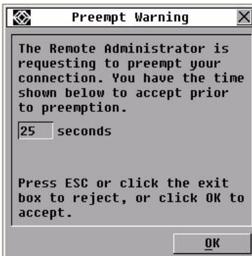
Figure 4-12. Preempt window
