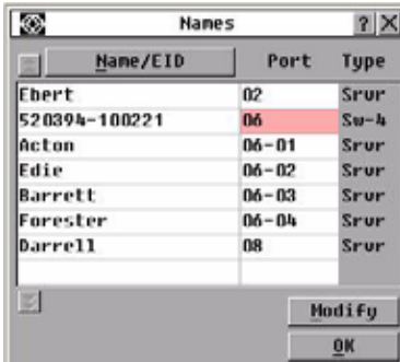
Figure 4-3. Names window
