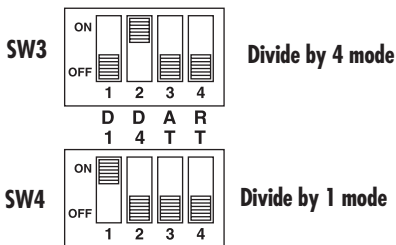
Figure 3-7. Clocking modes.
