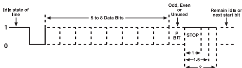
Figure D-1. Asynchronous communication bit diagram.
