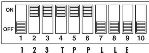
Figure 3-3. RS-485 4-wire with echo.
