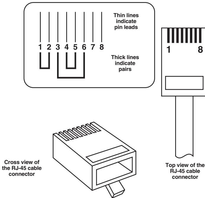
Figure 1-1. Active pair is pins 1 and 2, pins 4 and 5, or pins 3 and 6.
