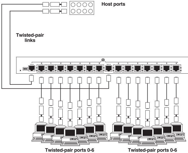
Figure 2-2. Networking the 5250 Star Repeater.
