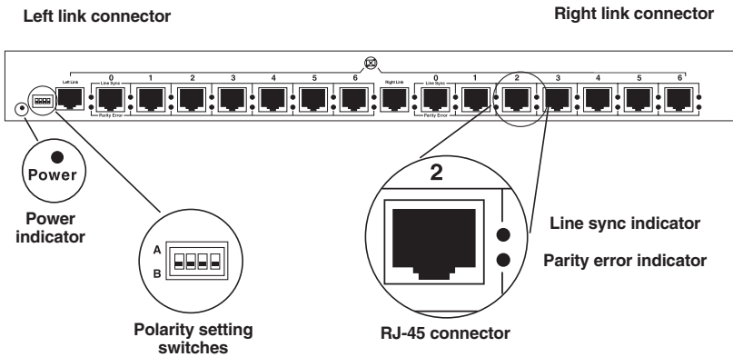
Figure 2-3. Connectors, switches, and indicators on the Repeater.
