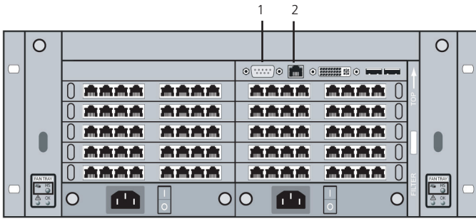
Figure 3-4. Front view, ACX080.
