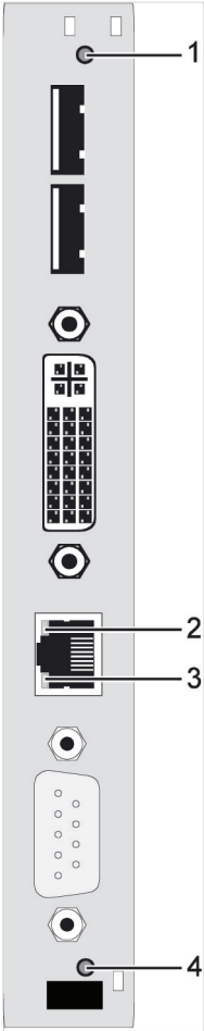
Figure 3-9. CPU board, front view.
