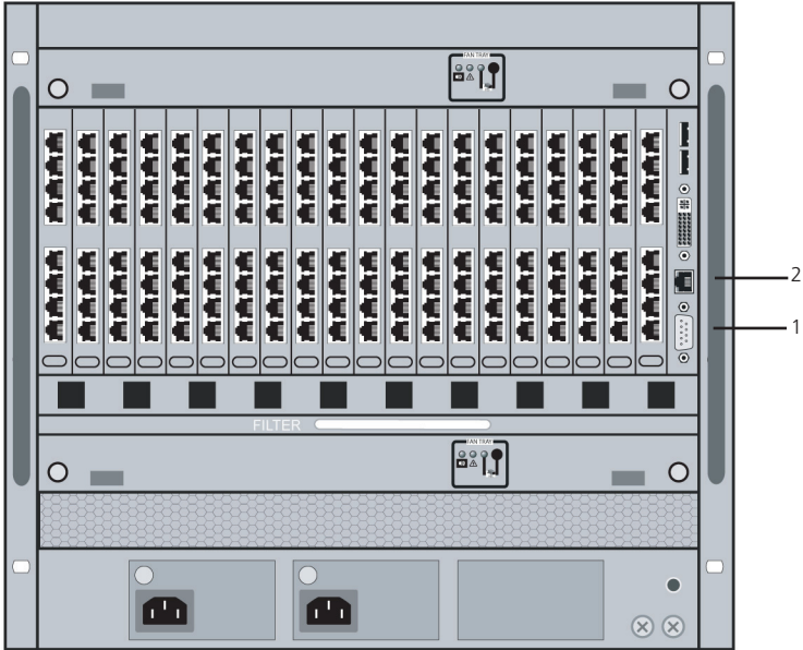
Figure 3-3. Front view, ACX160.
