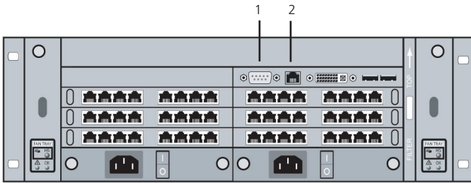
Figure 3-5. Front view, ACX048.
