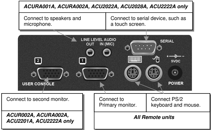
Figure 2 Single/Dual Head Remote Unit – rear view
