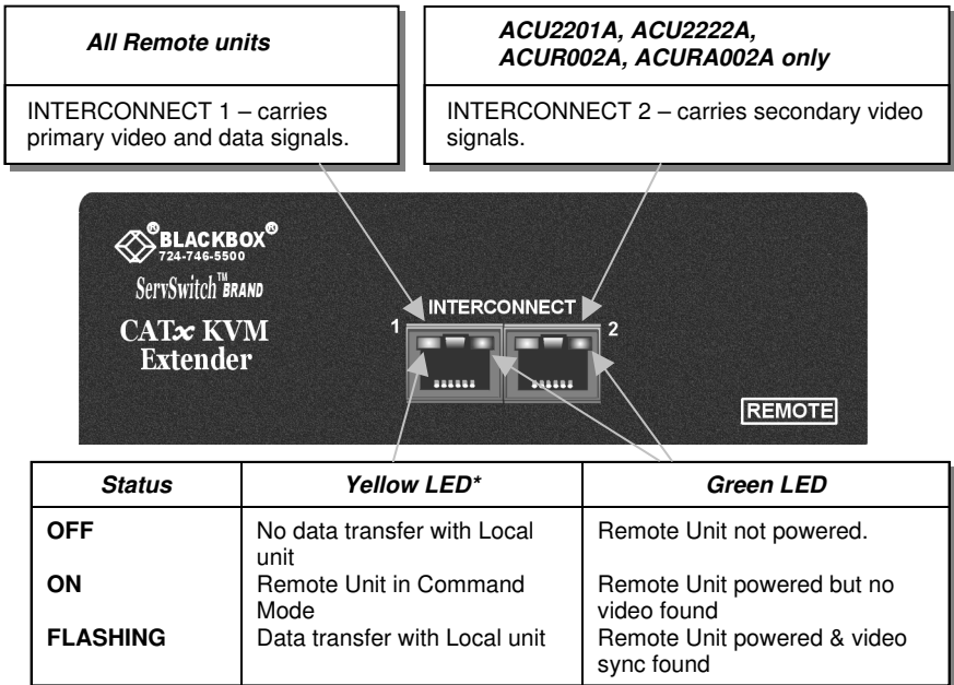
Figure 2 Single/Dual Head Remote Unit – rear view
