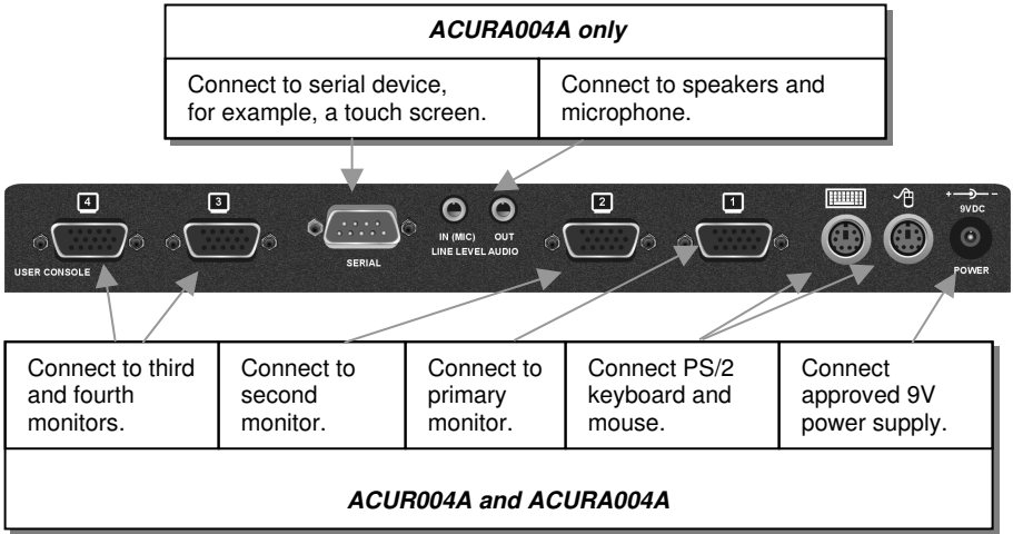
Figure 4 Quad Head Remote Unit – rear view
