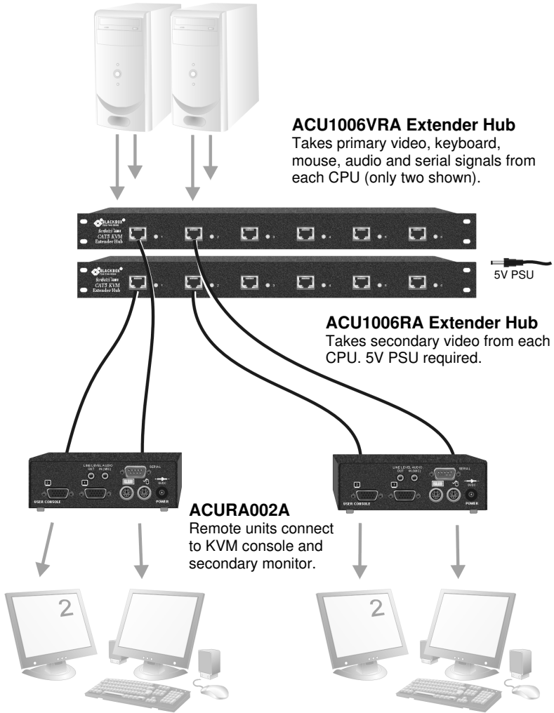
Figure 15 Dual-monitor consoles with serial and audio extension
