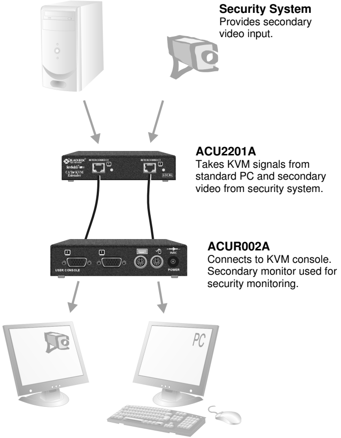
Figure 18 Extender system with second screen for security monitoring
