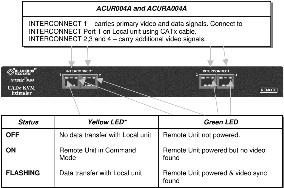
Figure 5 Quad Head Remote Unit – front view
