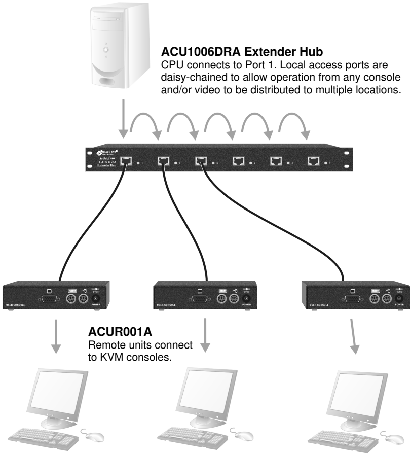
Figure 17 Information distribution system sharing a single PC
